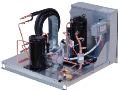
Next-Gen WC-Series Water Cooled Condensing Units 1/2 to 6 HP
