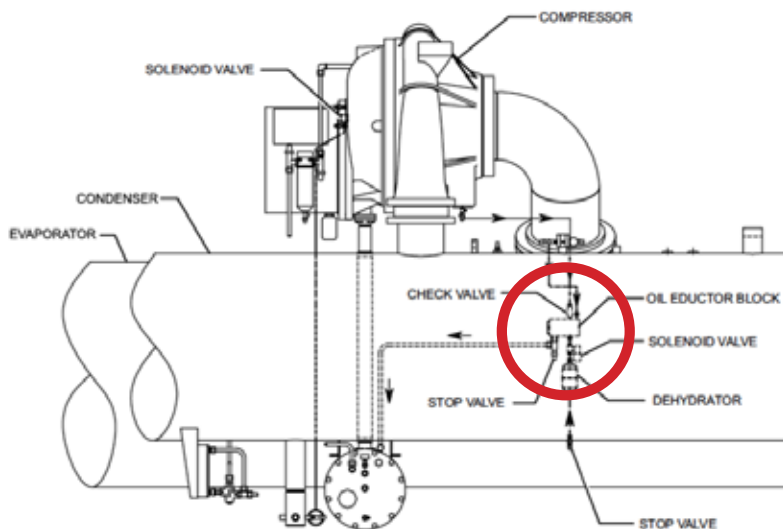
FIGURE 12 - OIL RETURN SYSTEM
